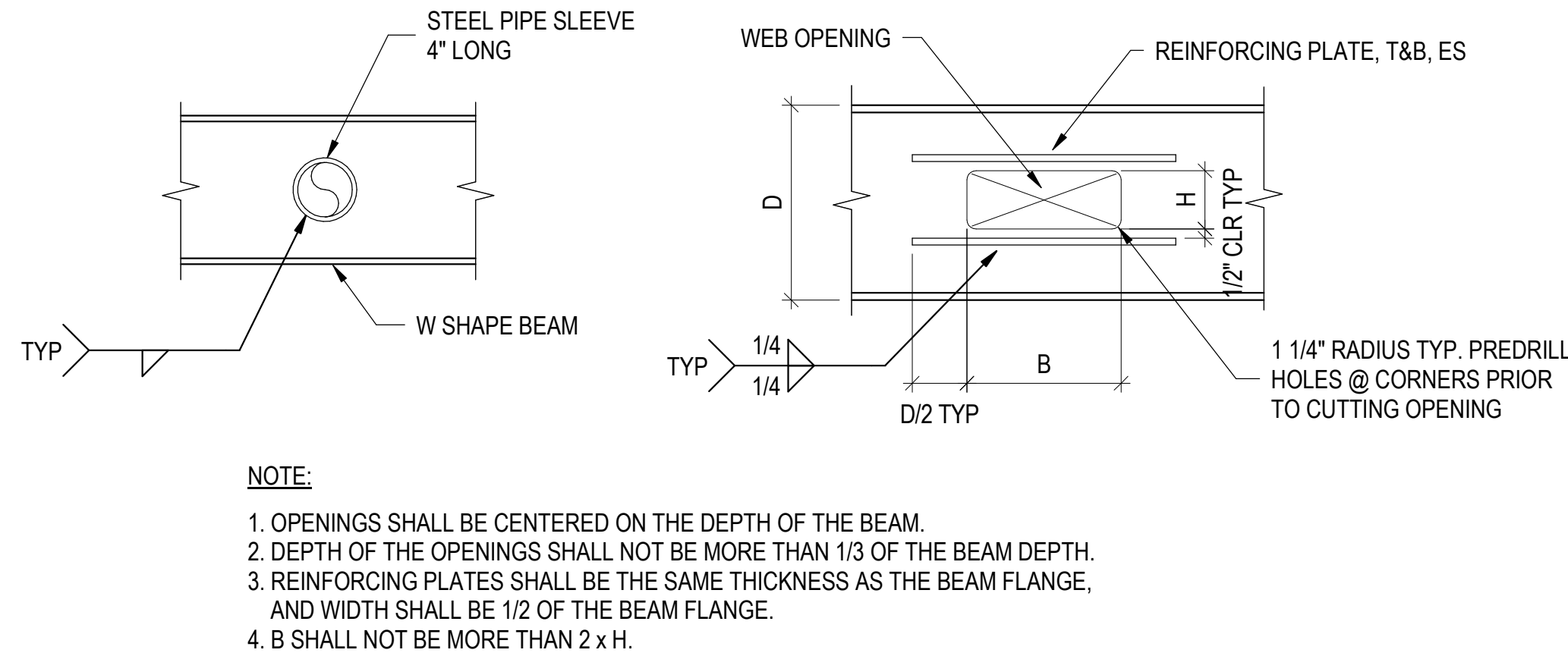
TYPICAL BEAM OPENING REINFORCING DETAIL
