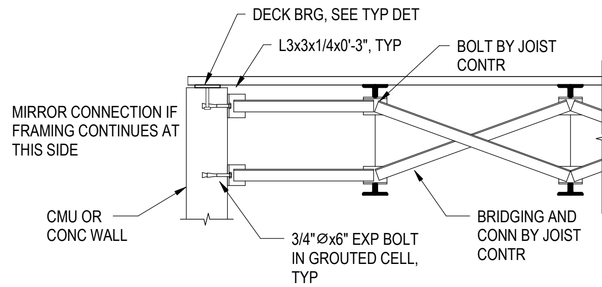
TYPICAL CROSS BRIDGING DETAIL
