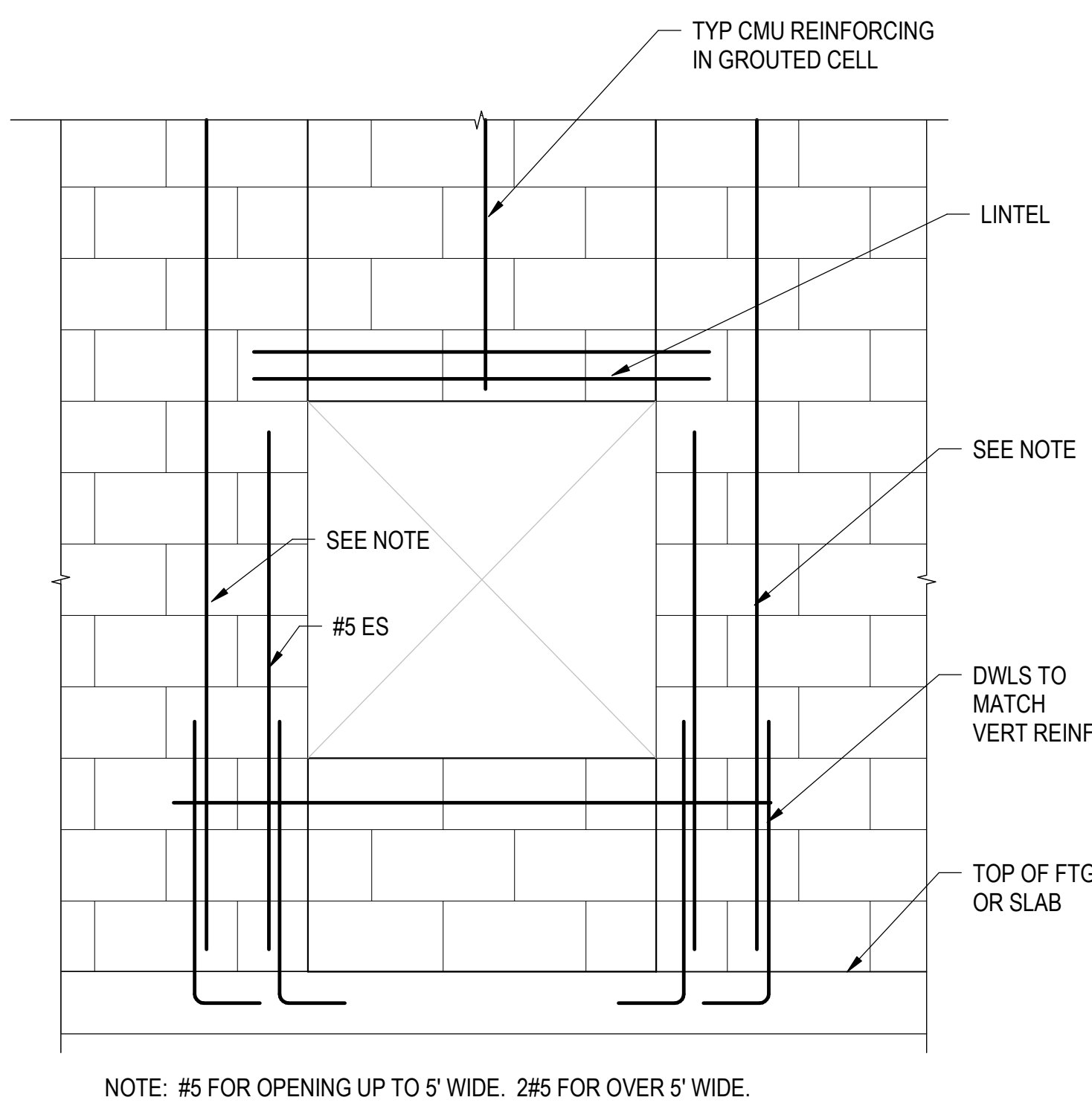
TYPICAL WALL REINFORCING AT CMU WALL OPNG DETAIL
