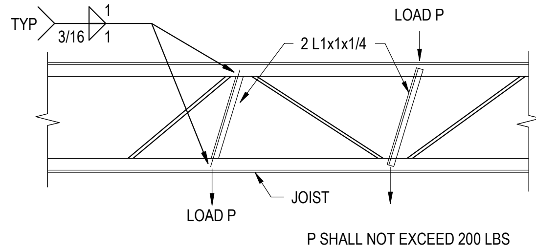
TYPICAL JOIST REINFORCEMENT DETAIL
